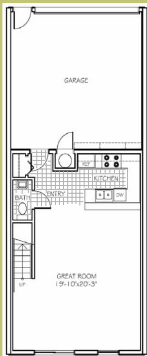
1st Floor
